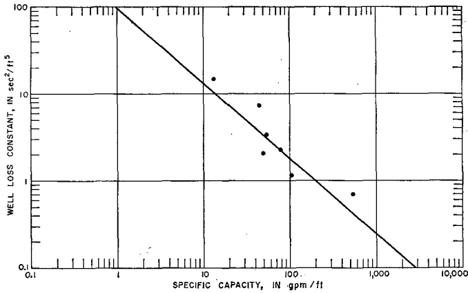
Fig. 48. Well-loss constant versus specific capacity, pumping levels are above the top of the Silurian dolomite aquifer.
