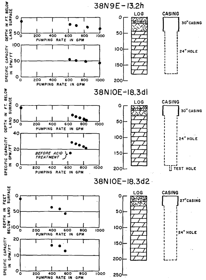
Fig. 47. Step-drawdown test data and construction features of wells 38N9E-13.2h, 38N10E-18.3d1, and 38N10E-18.3d2.
