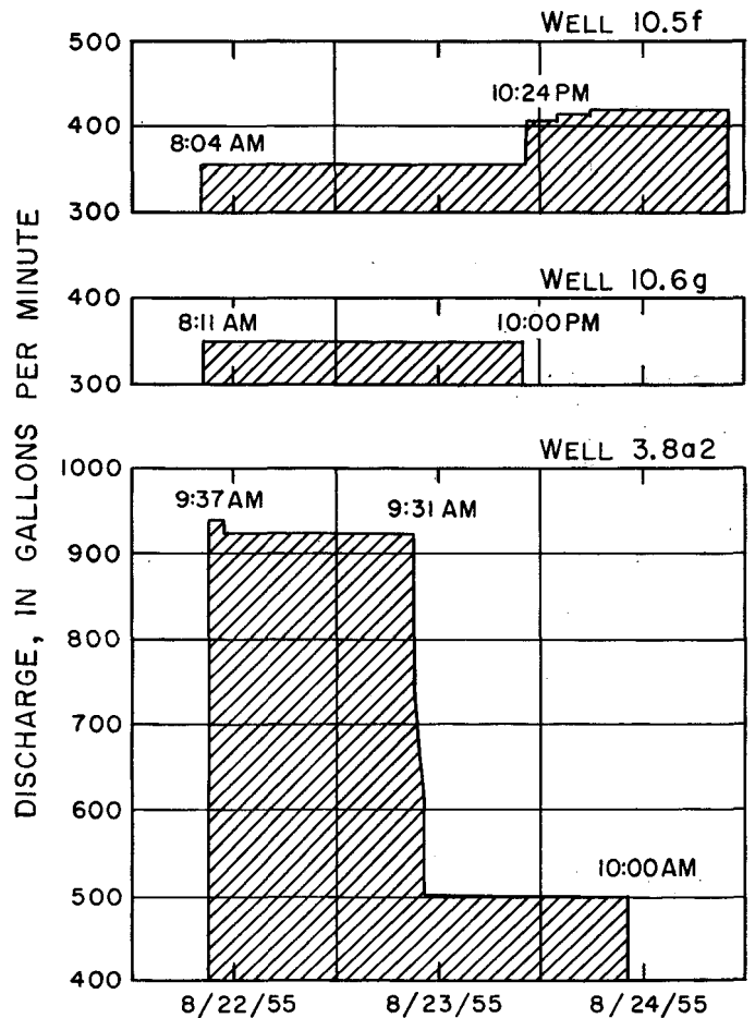
Fig. 41. Pumping conditions during pumping test 2.
