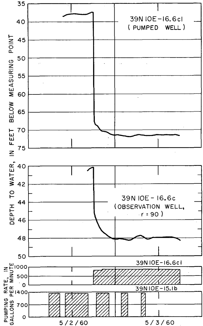
Fig. 37. Water levels and pumpage during pumping test 1.
