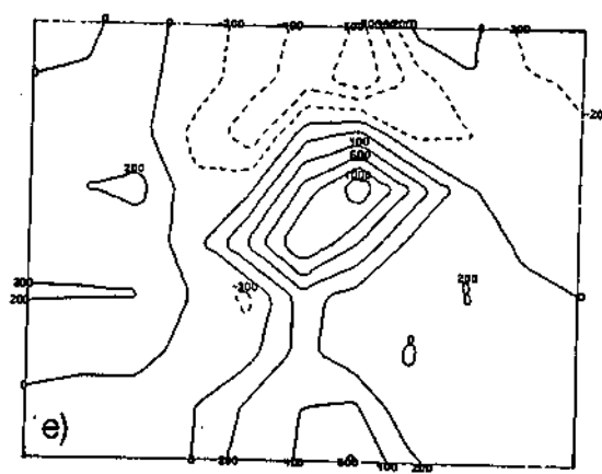
Figure B-27. Surface fields for the 5-min period beginning at 1910 CDT.
