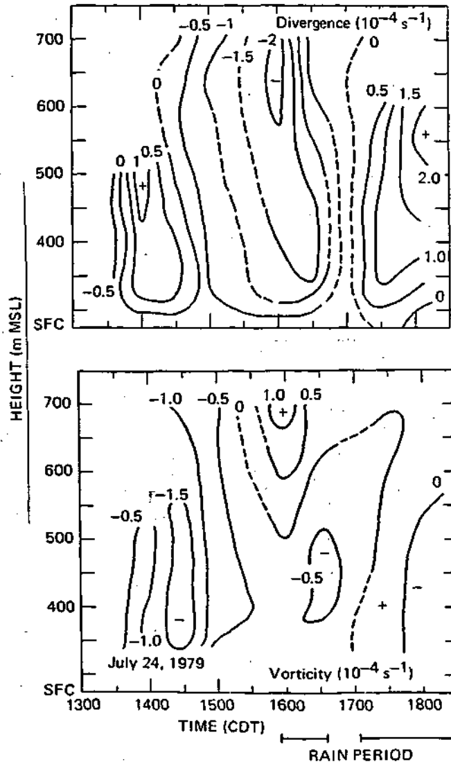
Figure 5. Time-height plot of divergence (top) and vorticity (bottom) in units 10^{-4} s^{-1} on 24 July 1979. Dashed lines indicate regions where measurements were sparse or lacking.
