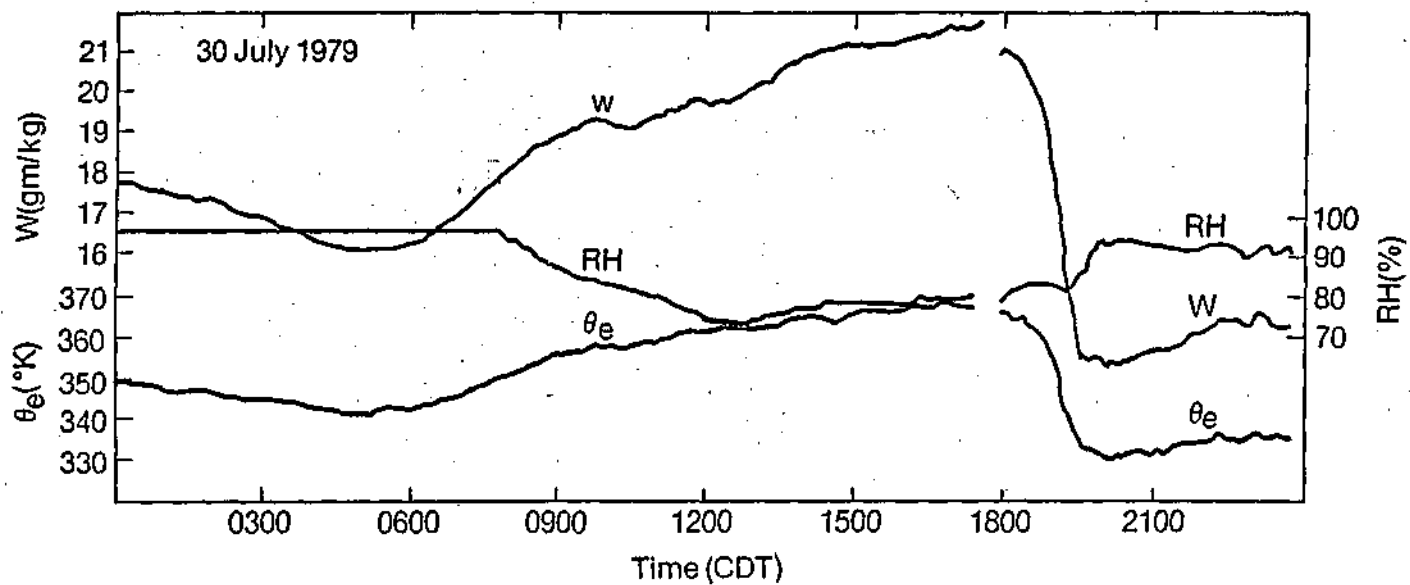
Figure B-17. Time profiles of area-averaged mixing ratio ( w ), relative humidity (RH) and equivalent potential temperature, \theta_e , based on one minute measurements at the 27 PAM stations.
