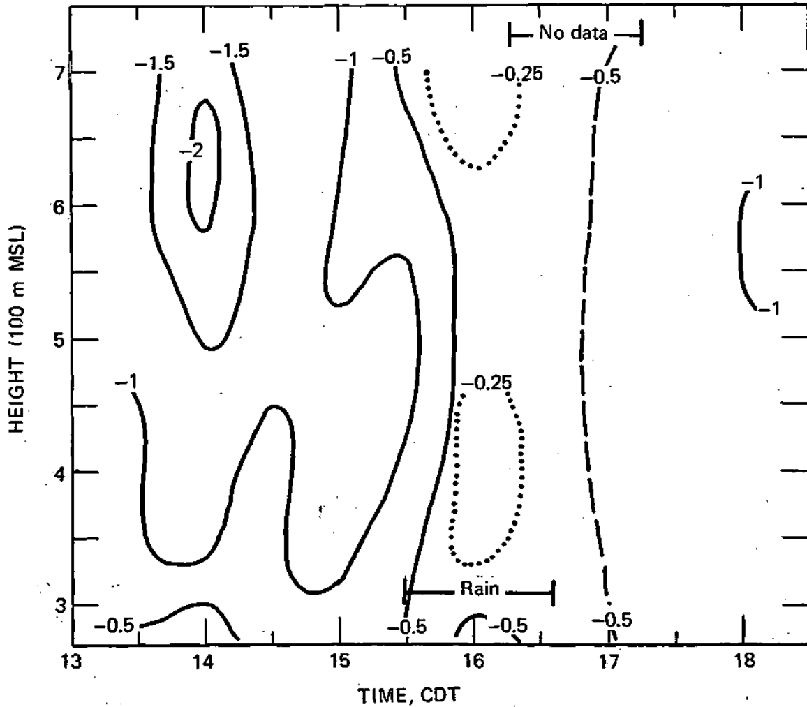
Figure B-42. Time - height cross-section of velocity divergence ( 10^{-4} \text{ s}^{-1} ) for triangular area defined by the three pilot balloon stations. Dashed contour is estimated because of missing data. Surface elevation is about 275 m MSL.
