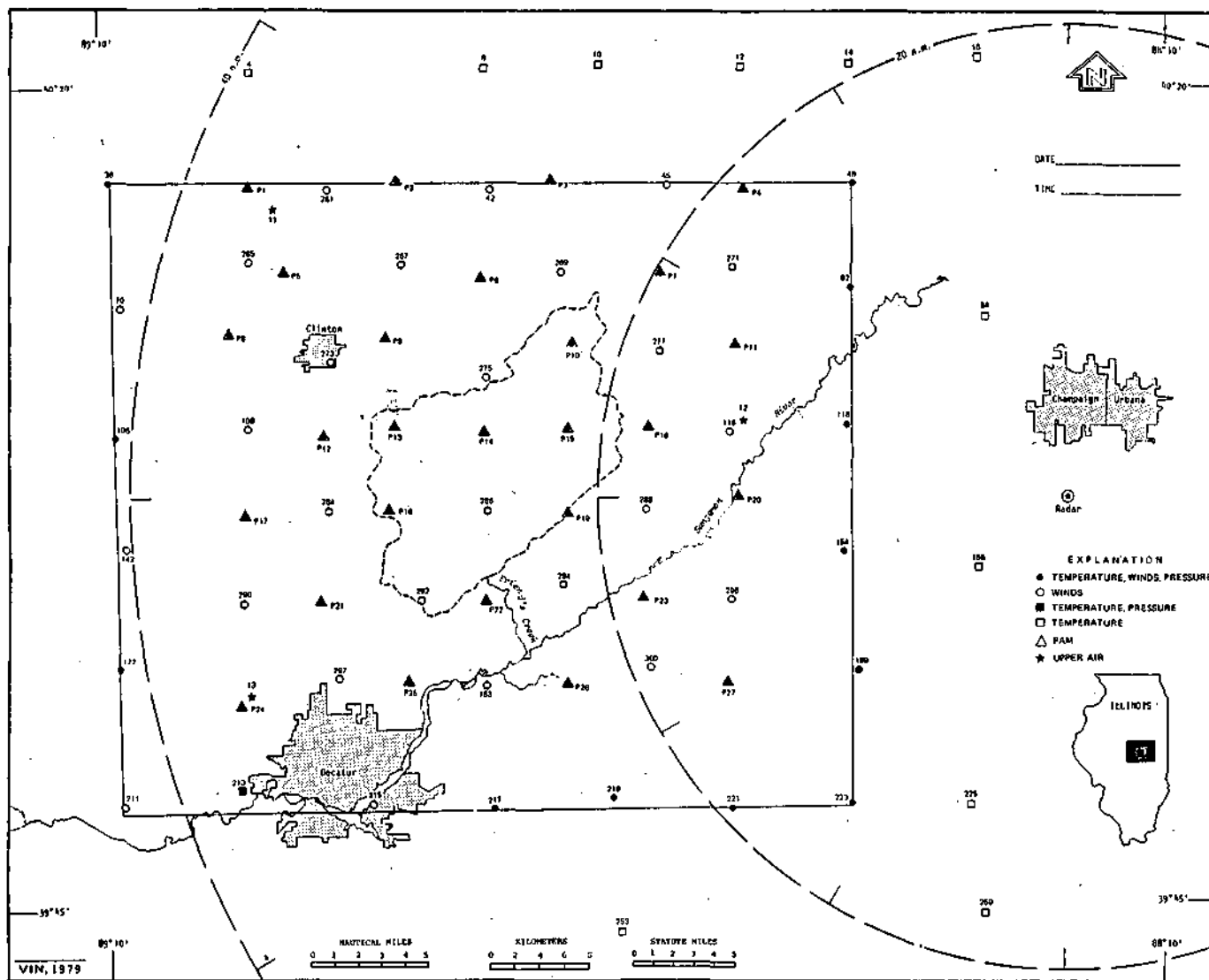
Figure 2. Surface wind network upper air stations and supplementary hygrothermograph/microbarograph stations. PAM stations are indicated by triangles. Pibal stations are shown by stars (numbered as station 11, 12 and 13).
