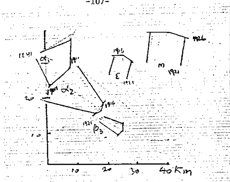
Figure B-39. Envelope at 40 dbz reflectivity contour (3.7° elevation). Tip of arrow indicates last location of detectable 40 dbz contour and direction of movement between times indicated. (See text for echo identification).
