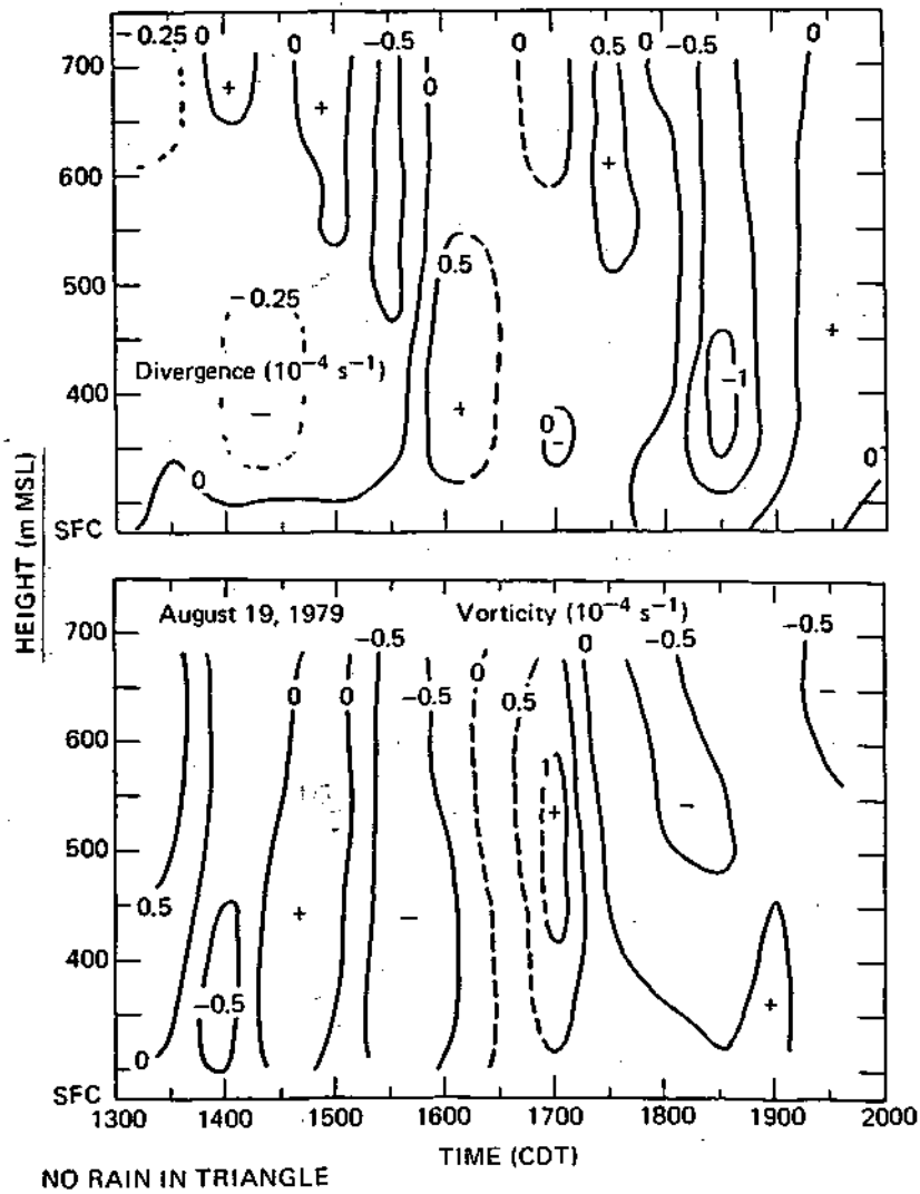
Figure 6. Time-height section of divergence (top) and vorticity (bottom) in units 10^{-4} s^{-1} on 19 August 1979. The short-dashed lines are intermediate contours, the long dashes indicate regions where measurements were lacking.
