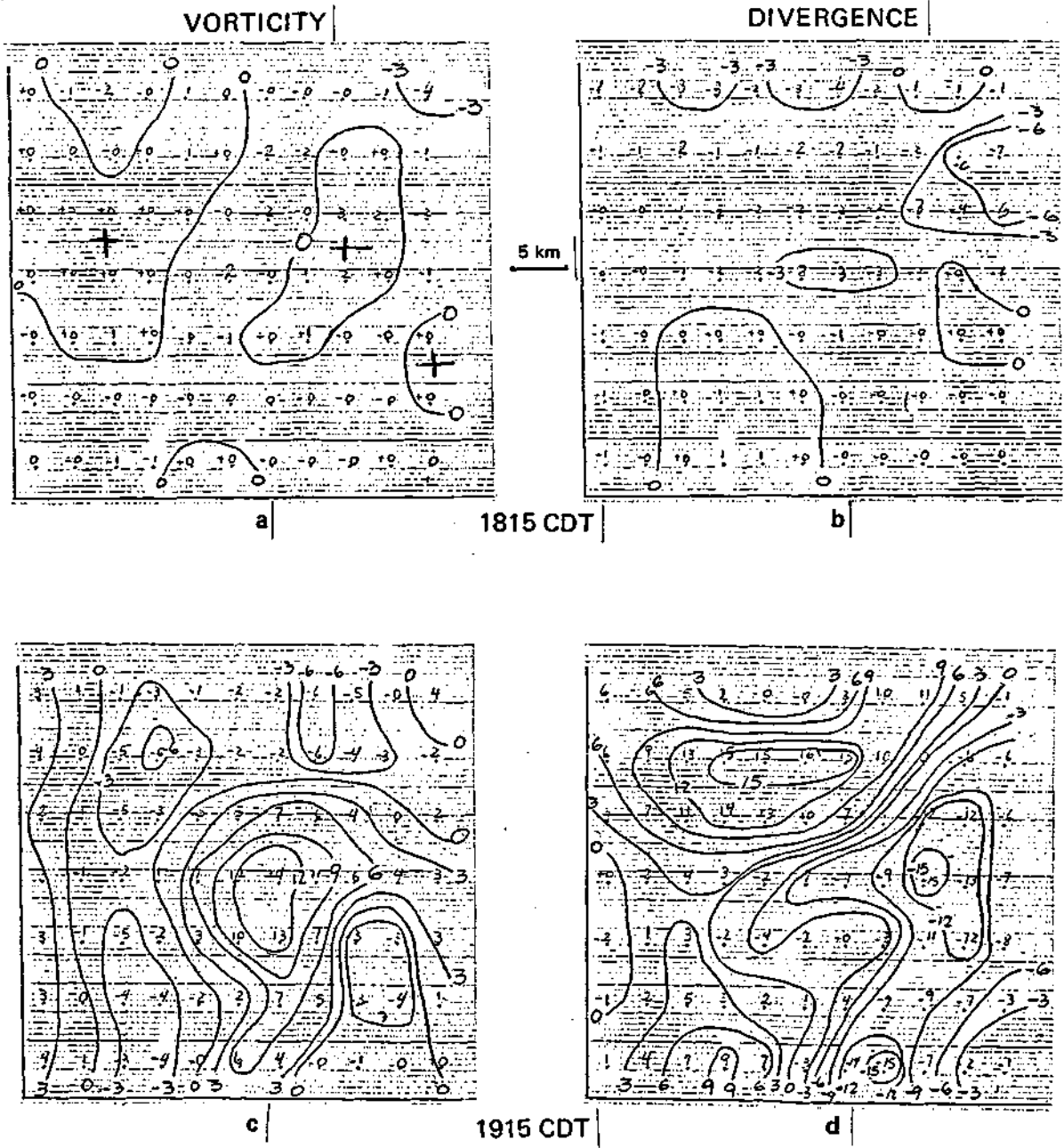
Figure B-36. Vorticity and divergence in inner weather network at 1815 CDT (a,b) and 1915 CDT (c,d). Units are 10^{-4} \text{ s}^{-1} .
