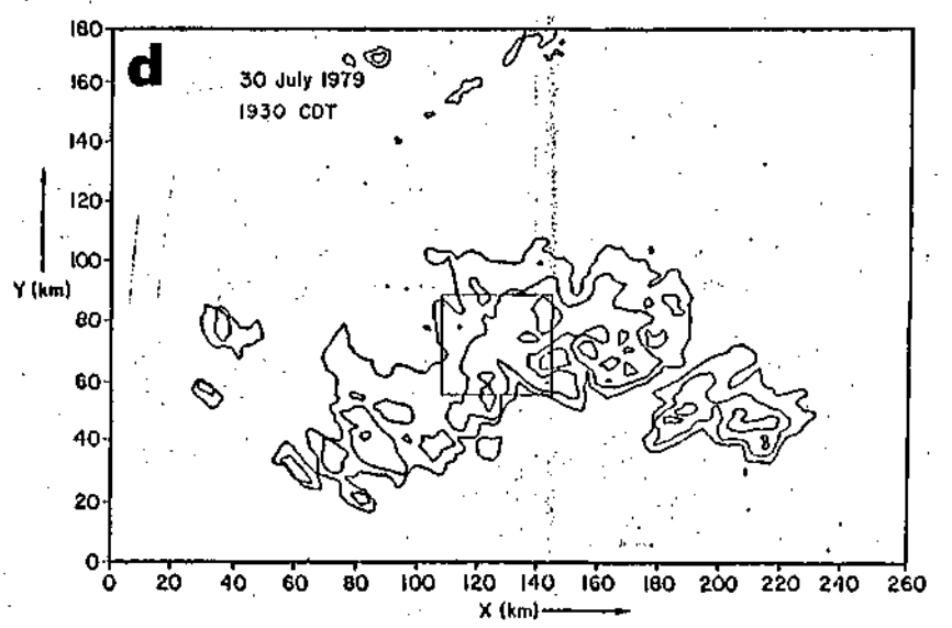
Figure B-32, Contoured echoes detected by SWS HOT radar at Joliet. Box indicates location of the VIN network.
