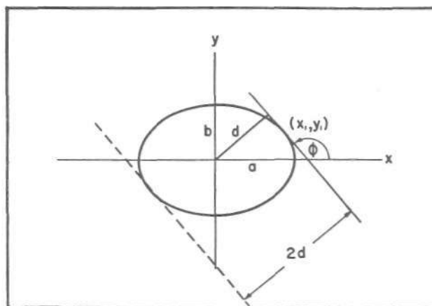
FIG. 4. Prolate ellipsoid of revolution.
