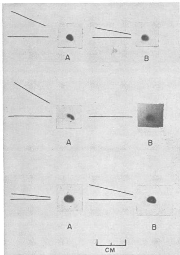
FIG. 3. Photographs of raindrops from two angles.
