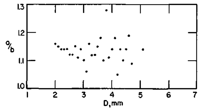
FIG. 9. Average prolate raindrop axial ratio.
