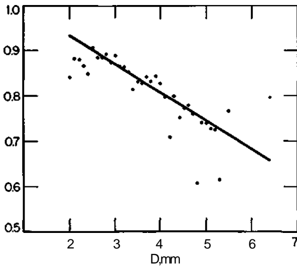
FIG. 8. Average oblate raindrop axial ratio.
