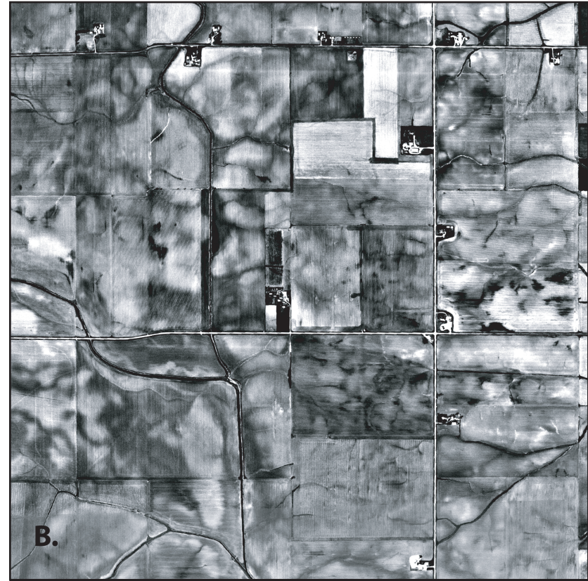
Figure W2. (A) Portion of July 30, 1939 airphoto of confluence of Senachwine Creek and northern tributary in glacial lake plain. Some reaches showed signs of alteration, but the mainstem was free flowing. Image obtained from ISGS Historical Airphoto Archive. (B) The same area in 1998. Senachwine Creek was completely altered by this time. Image is a USGS DOQ.
