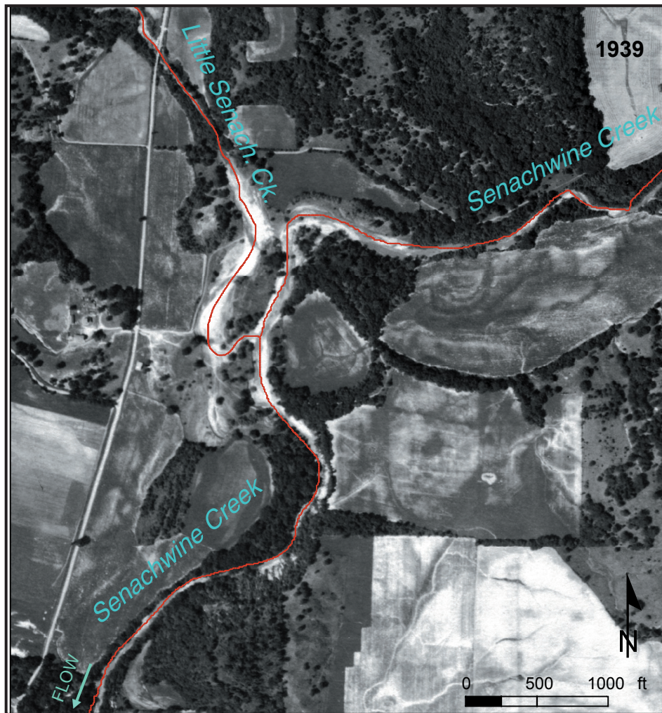
Confluence of Little Senachewine Creek and Senachewine Creek, extreme NE Peoria County, in 1939 (left) and 1998 (right). Little Senachewine shows little change, but the confluence was pirated by downstream migration of a Senachewine Creek meander. Other meanders show mainly downstream migration of 300-500 ft (5-8 ft/yr) over the period. The main change in the landscape was increased density of the forest cover on high sloping areas and along drainages, and a more continuous riparian forest cover. Flow is towards bottom of page.
