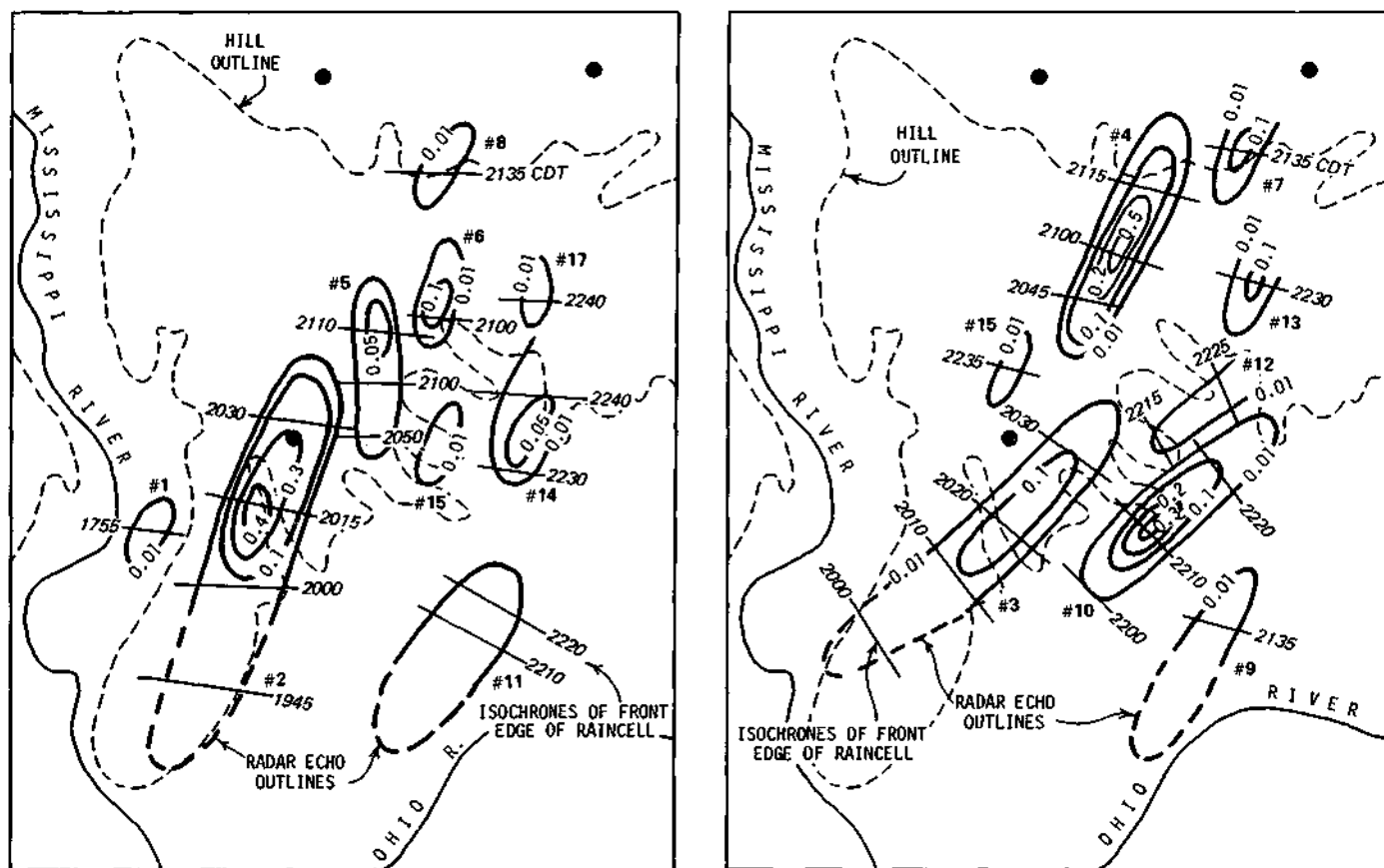
Figure 20. Raincells on 26 July 1970
