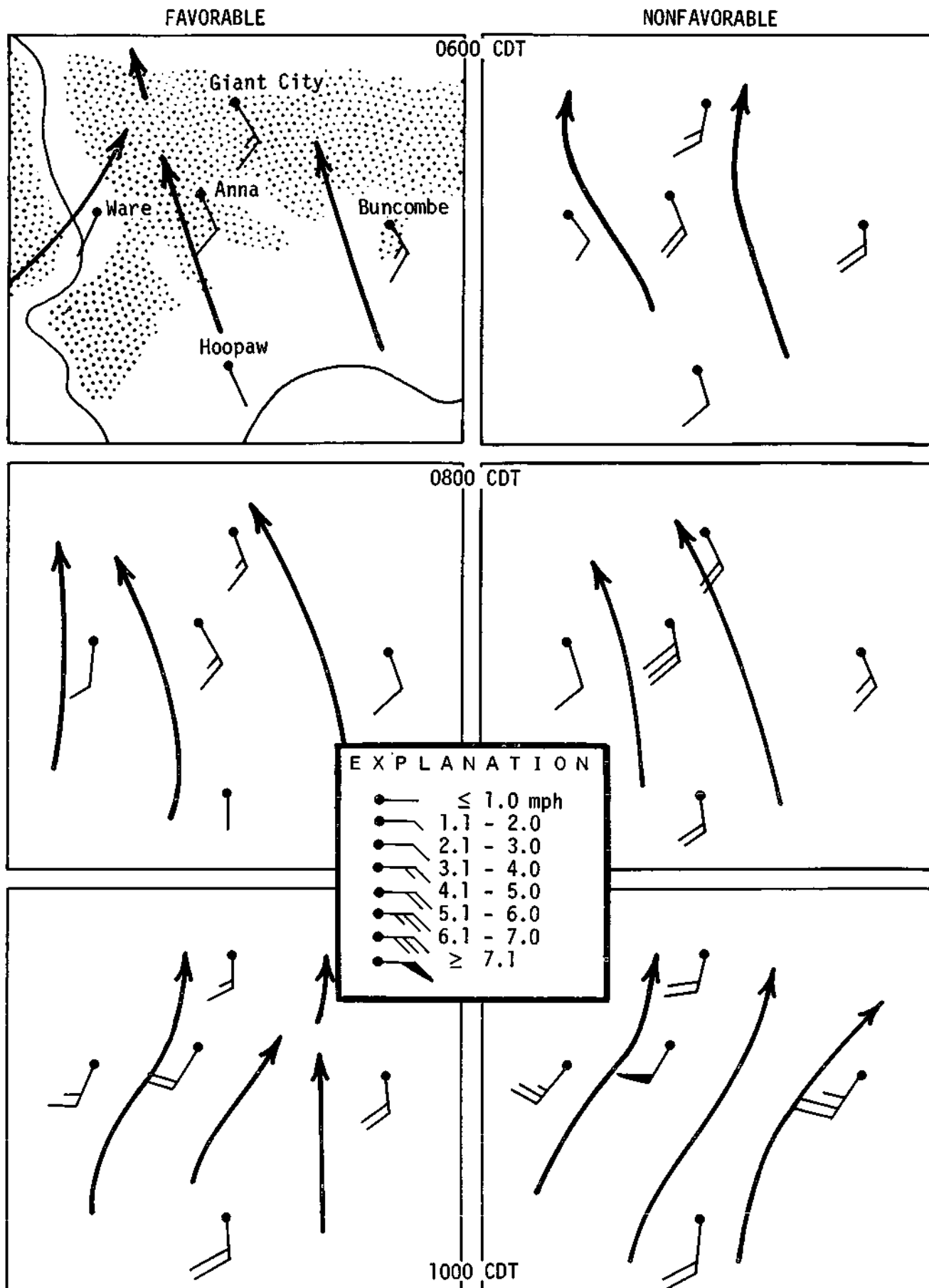
Figure 33. Prevailing winds and average speed, mph, on favorable and nonfavorable days
