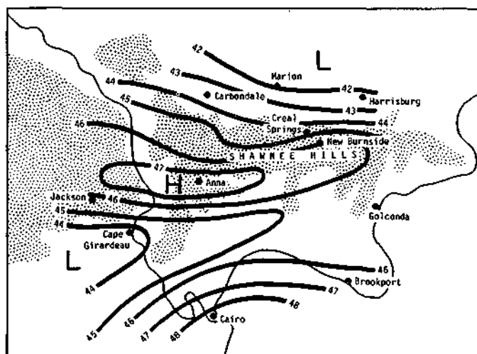
Figure 3. Adjusted average annual precipitation, inches, 1931-1967
