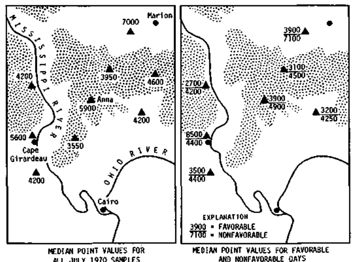
Figure 28. Median CCN values at airborne sampling locations
