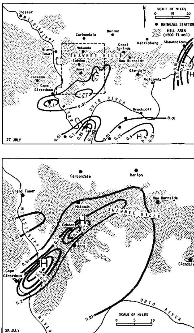
Figure 21. Rainfall, inches, on 27-28 July 1970
