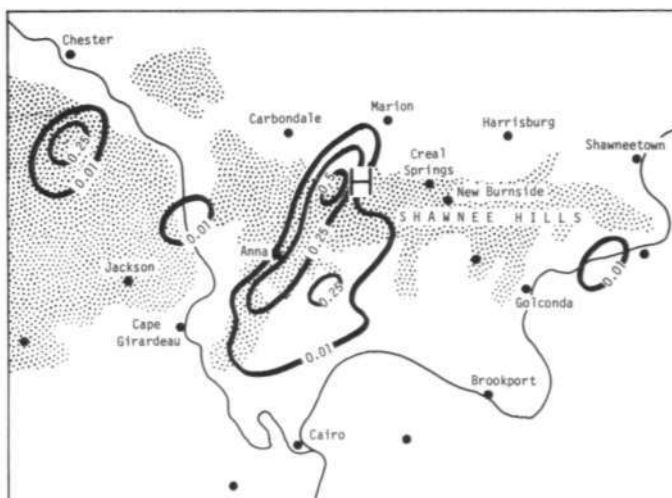
Figure 19. Rainfall, inches, on 26 July 1970
