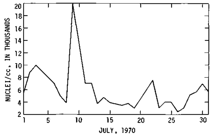
Figure 27. Median values of CCN on each flight in July 1970
