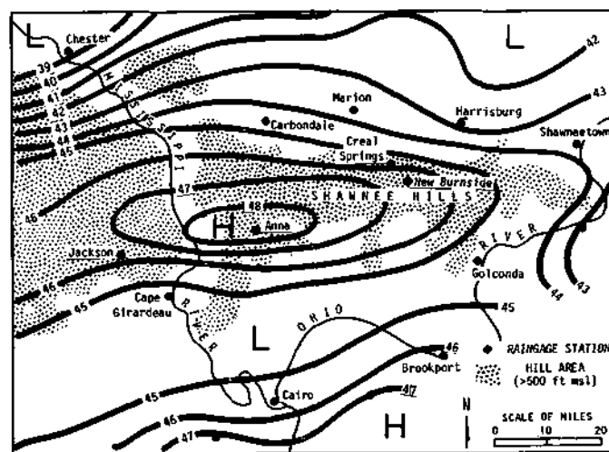
Figure 1. Average annual precipitation, inches, 1931-1960
