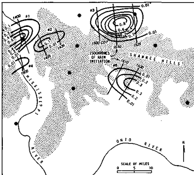
Figure 24. Raincells on 31 July 1970
