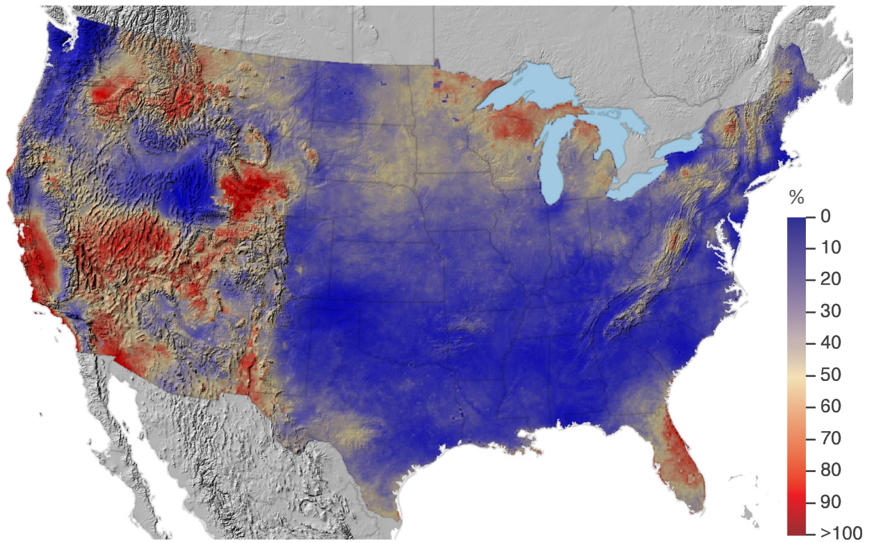
Annual chloride deposition in 2015 (top), and percentage of total chloride deposition as dry deposition in 2015 (bottom).
