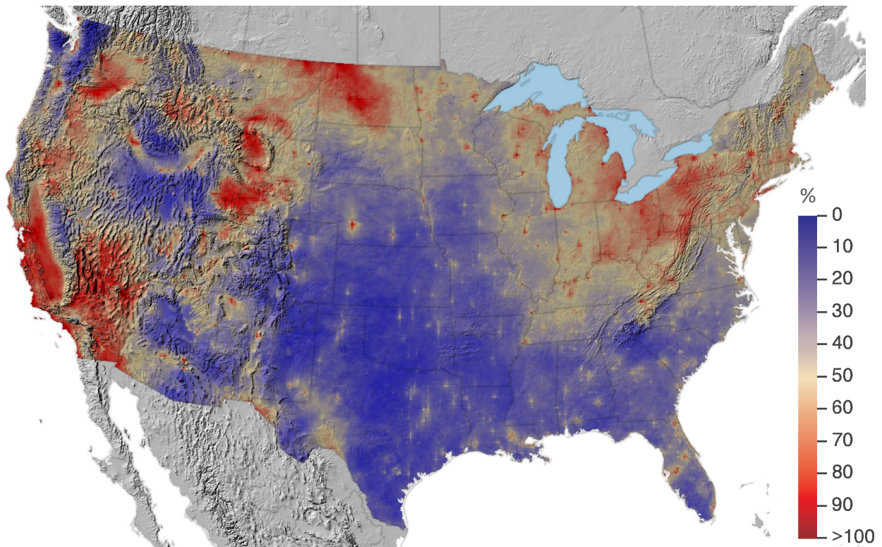
Annual sulfur deposition in 2015 (top), and percentage of total sulfur deposition as dry deposition in 2015 (bottom).
