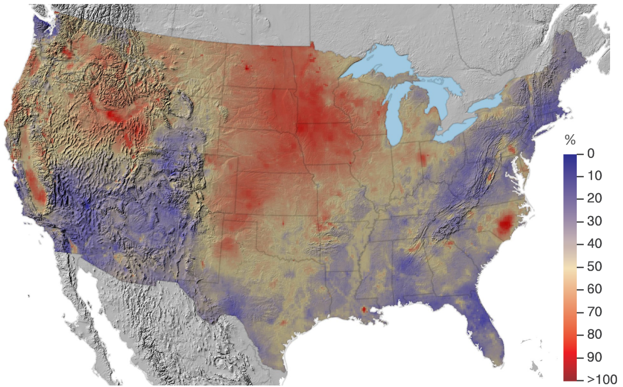
Annual reduced nitrogen deposition in 2015 (top), and percentage of total nitrogen deposition as reduced nitrogen in 2015 (bottom).
