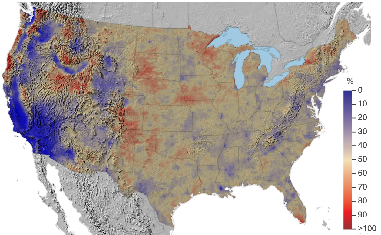
Annual wet nitrogen deposition in 2015 (top), and percent of total nitrogen deposition as wet deposition in 2015 (bottom).
