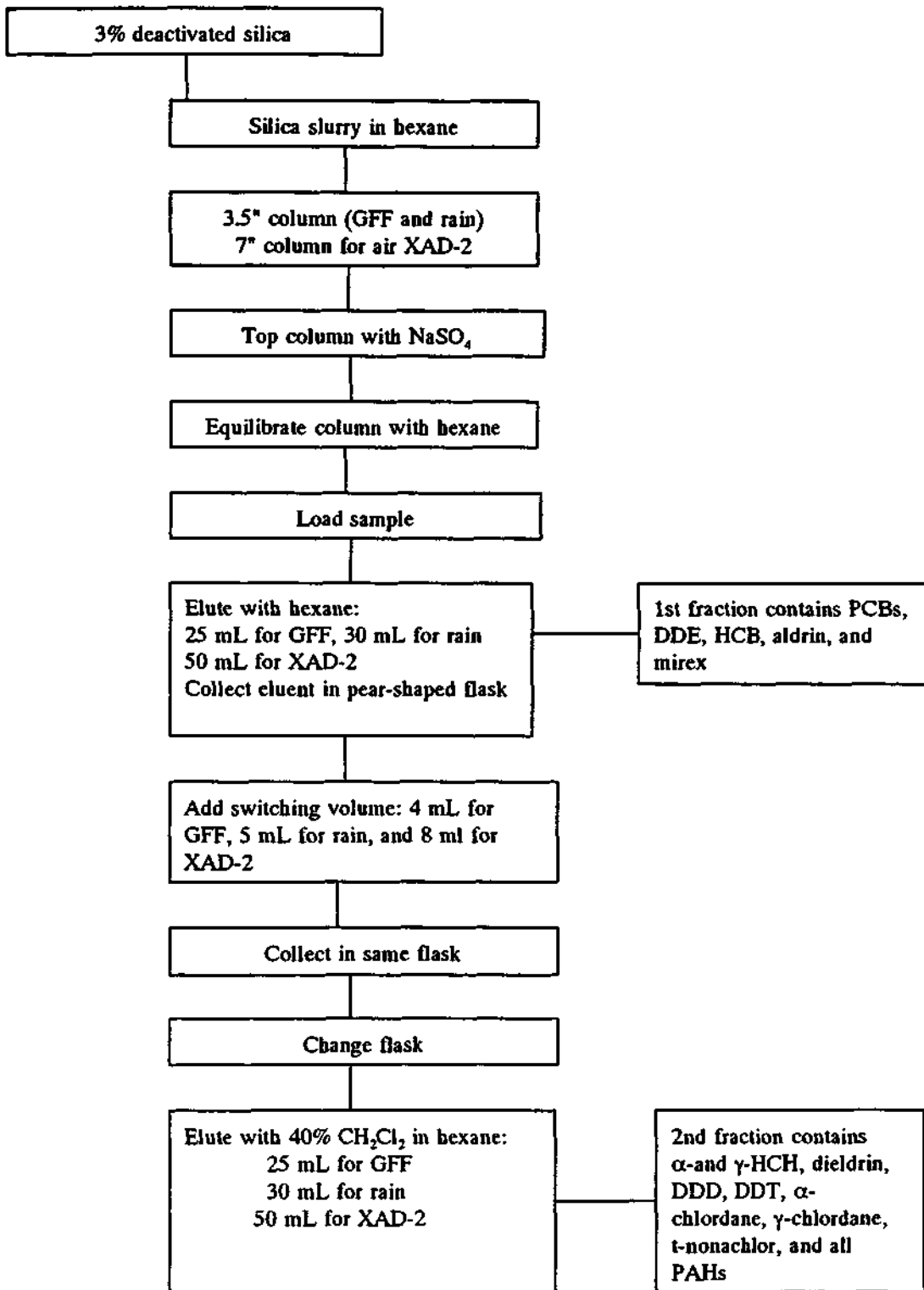
Figure 7. Procedure for Silica Column Chromatography Separation
