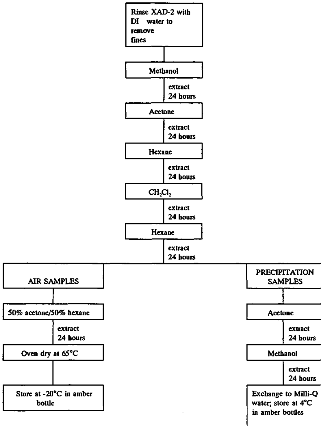
Figure 4. Flowchart of XAD-2 Precleaning Procedure
