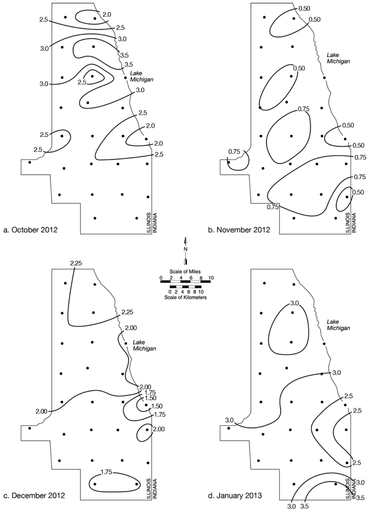
Figure 5. Precipitation pattern (inches) for October 2012–September 2013
