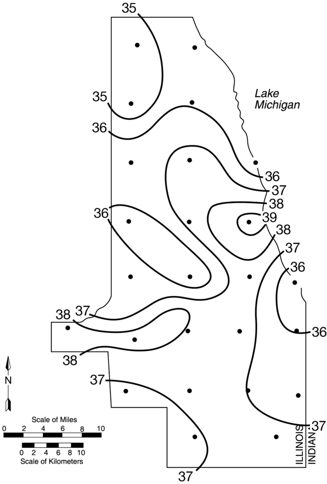
Figure 6. The 24-year average precipitation pattern (inches), Water Years 1990–2013
