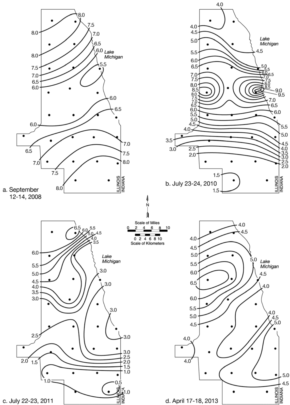
Figure IV-1. The four most intense storm events during Water Years 2008-2013.
