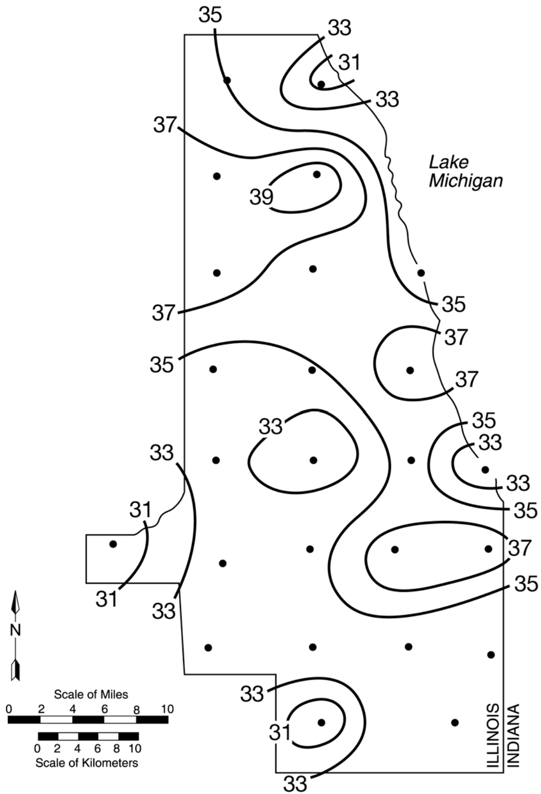
Figure 3. Precipitation pattern (inches) for Water Year 2013
