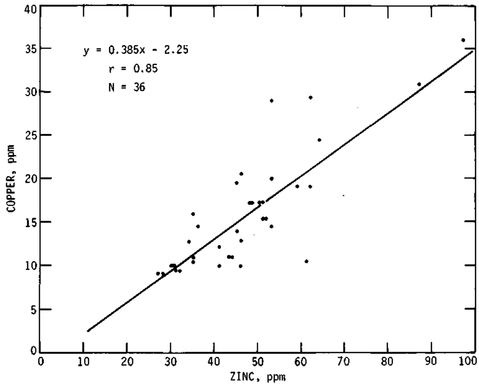
Figure 31. Relationship of copper and zinc in soils
