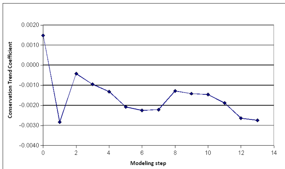
Figure B.6: Effects of binary site variables and spike dummies on estimated coefficient of conservation trend variable.
