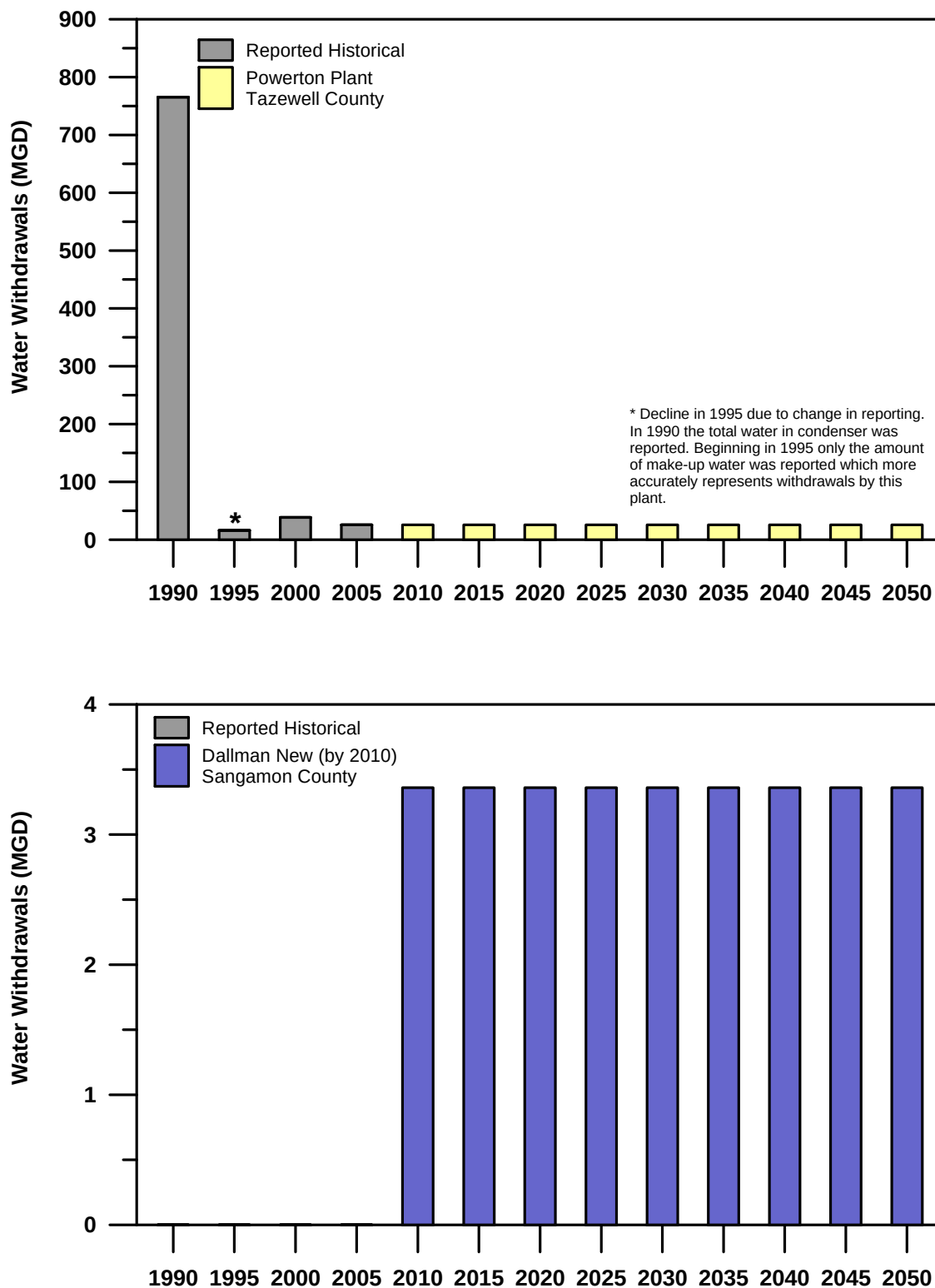
Figure 3.5: Historical and future power generation water withdrawals from the baseline scenario for the Powerton and Dallman (new) plants.
