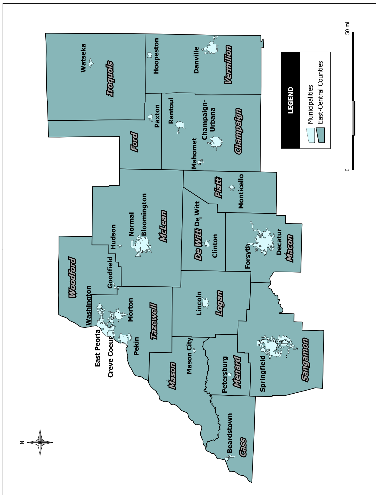
Figure 2.1: Map of 26 public water supply study areas modeled in addition to the 15 counties within the East-Central Region.
