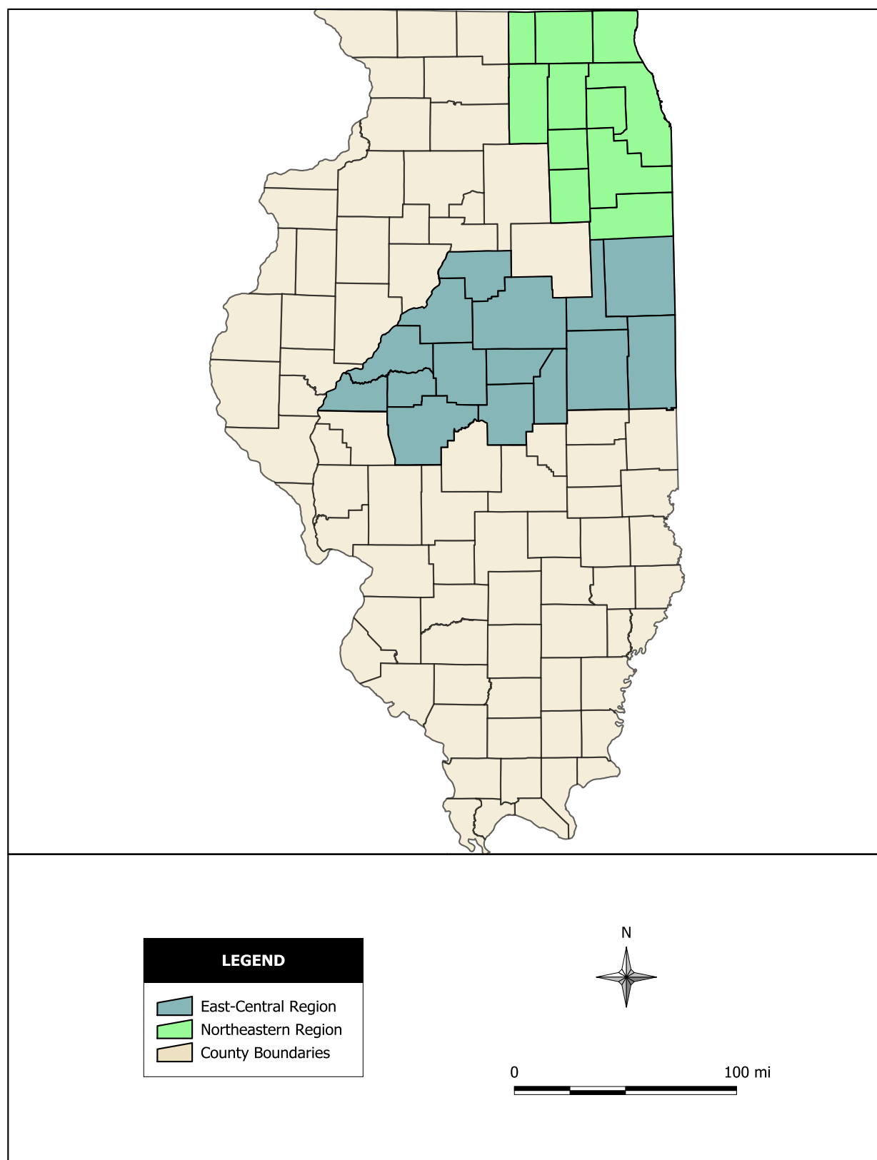
Figure 1.1: The two priority planning regions in Illinois identified through work by the Illinois State Water Survey.
