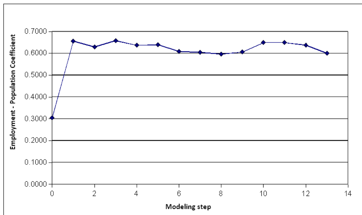
Figure B.5: Effects of binary site variables and spike dummies on estimated coefficient of population to employment ratio.
