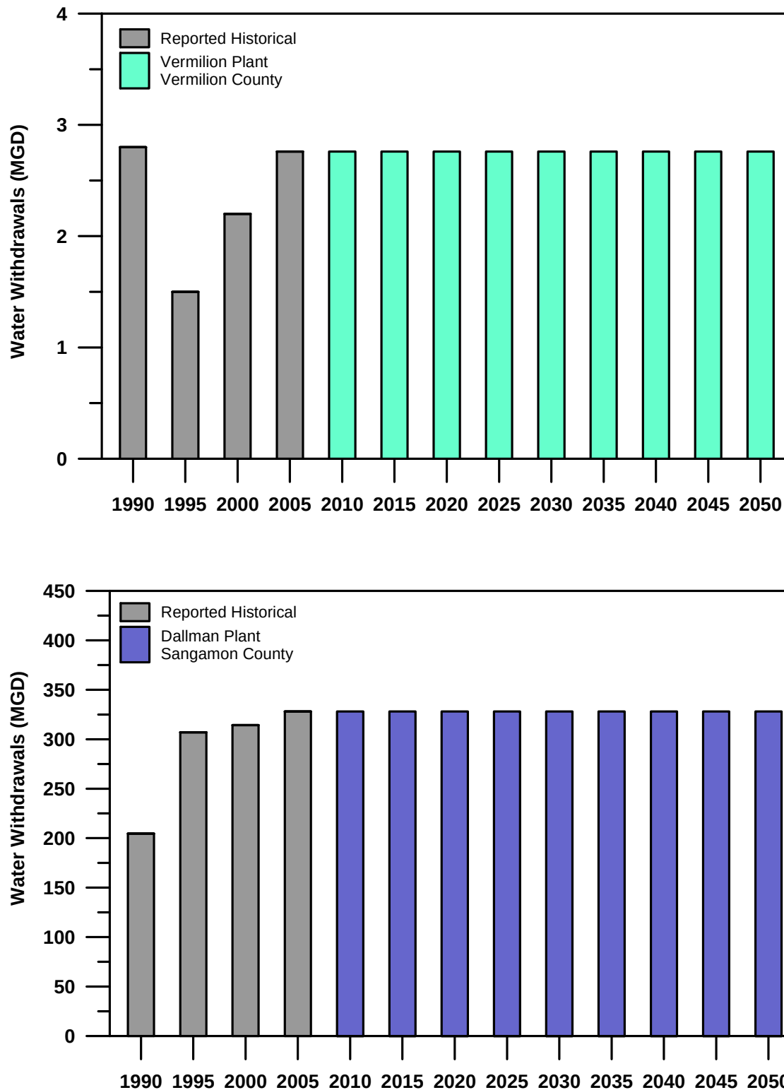
Figure 3.6: Historical and future power generation water withdrawals from the baseline scenario for the Vermilion and Dallman (existing) plants.
